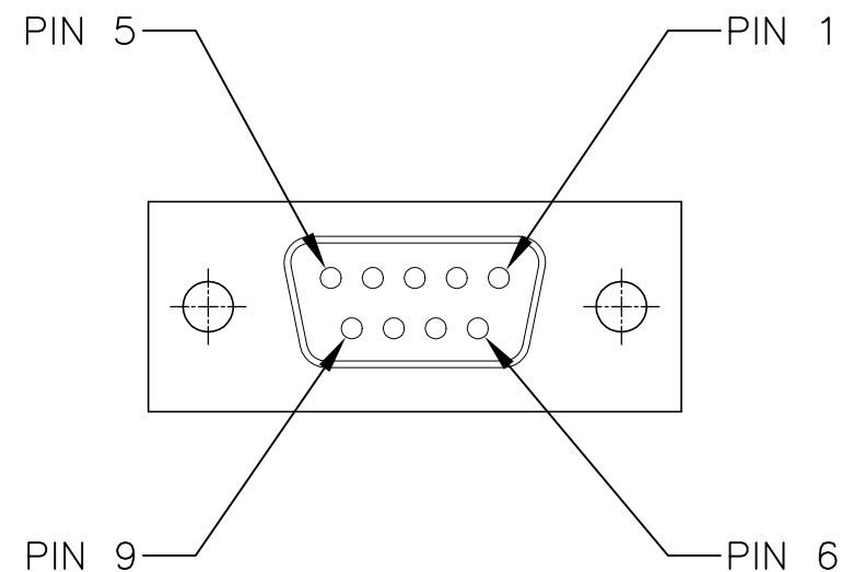
FEMALE DB-9
